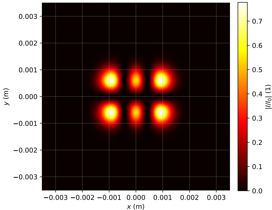
Intensity profile I(x, y, z = 1.274)/I_0 , P_{in}=0.5P_{cr} , artificial time
